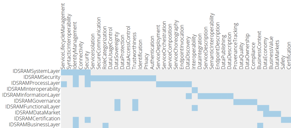
Figure 10. IDS Classifications with related concerns.
