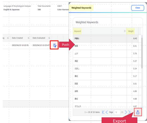
Figure 5: One of the features to be released in the next version of KAM that is designed to help identify key words and review documents
