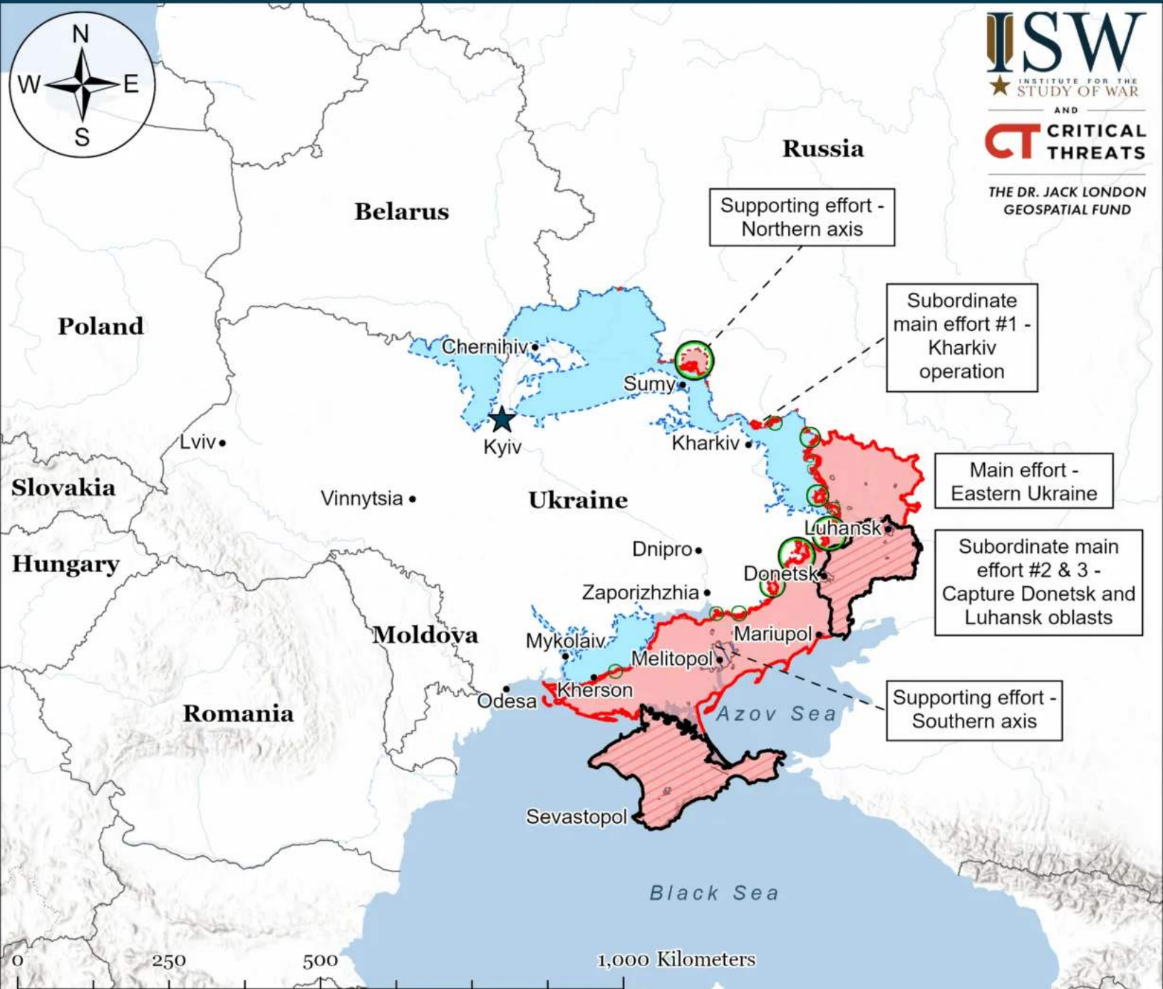
Map by George Barros, Kateryna Stepanenko, Daniel Mealie, Harrison Hurwitz, Derik Durbin, Benjamin Cordola, David Schulert, Quinn Deutschendorf, Lea Corticchiato, Megan Ewert, Nathaniel Kramer, and Carolyn Weinstein © 2025 Institute for the Study of War and AEI's Critical Threats Project
